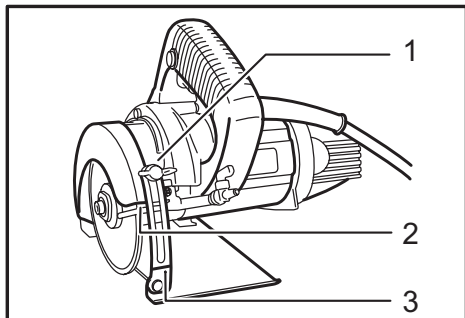
► 1. Wing bolt 2. End of blade case 3. Red line
