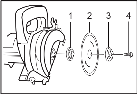
► 1. Inner flange 2. Diamond wheel 3. Outer flange 4. Hex socket head bolt
