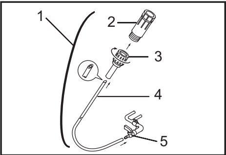
► 1. Pressure regulator assembly 2. Pressure regulator 3. Adapter 4. Vinyl tube 5. Water pipe
