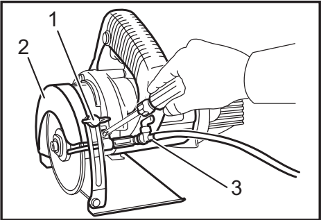
► 1. Wing bolt 2. Blade case 3. Water pipe
